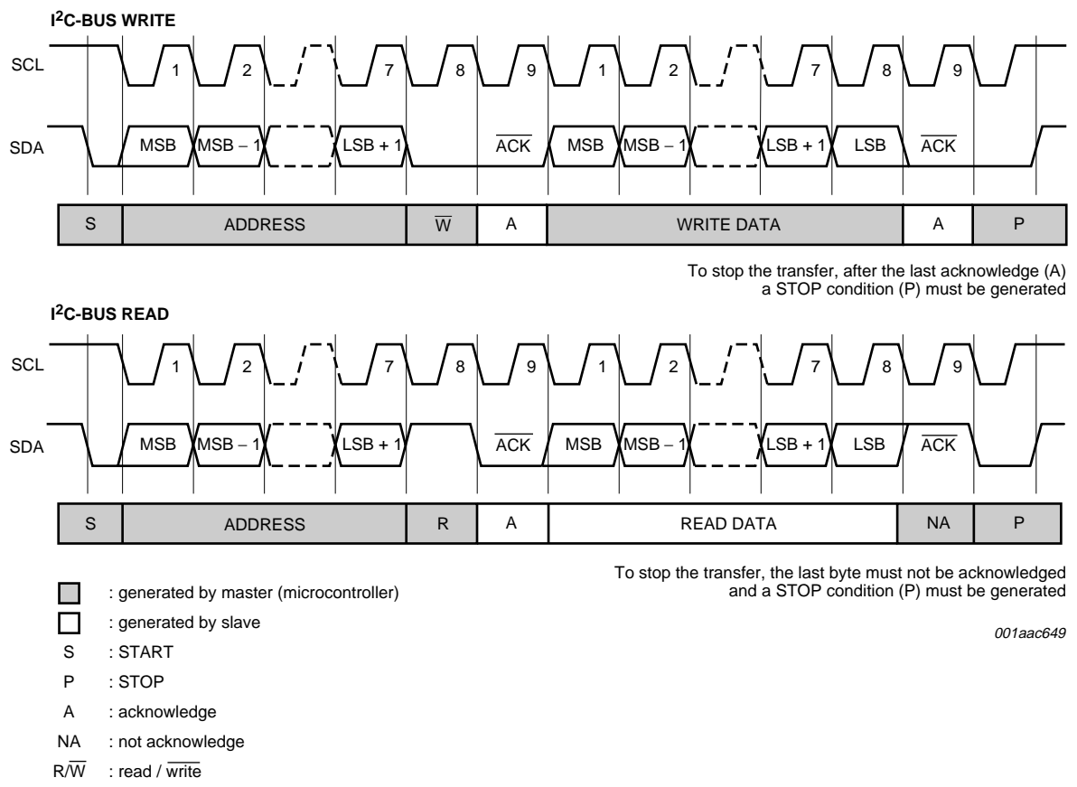
Fig 17. I 2 C-bus read and write modes
